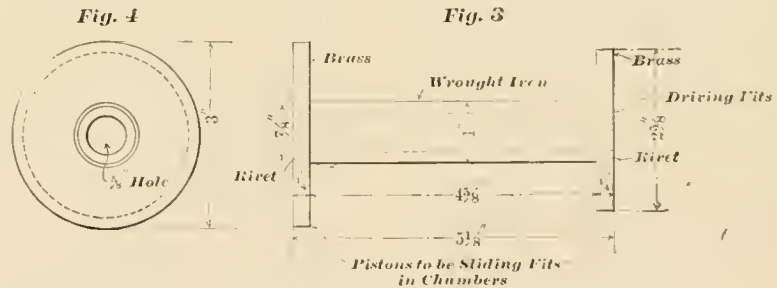
AUTOMATIC AIR PUMP DRAIN—DETAILS OF PISTON PARTS.
